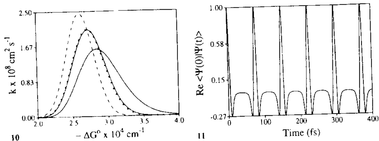
Fig. 10. Rate constant as a function of -\Delta G^0 for the \text{Fe}^{\text{III}}(\text{H}_2\text{O})_6/\text{Ru}^{\text{II}}(\text{NH}_3)_6 cross reaction where the two solvent modes are treated as harmonic while the metal ligand modes are characterized by varying degrees of anharmonicity. Dashed: \delta = 0 (harmonic-no anharmonicity); dotted: \delta = 1 ; and right hand solid curve: \delta = 2 . Left hand solid curve employs \delta = 1 for the low-frequency metal ligand mode and \delta = 2 for the high frequency mode in the \text{Fe}^{\text{III}}/\text{Fe}^{\text{II}} and \text{Ru}^{\text{II}}/\text{Ru}^{\text{III}} couples
