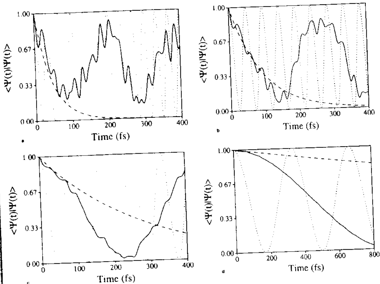
Fig. 13. Survival probability of the population on the reactant electronic surface for the one-mode system with potential couplings from top to bottom of 500, 350, 200, and 50 \text{cm}^{-1}
