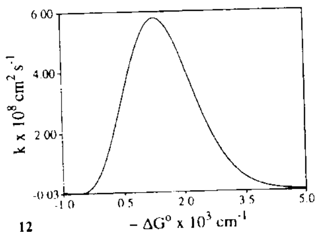
Fig. 12. Rate constant as a function of -\Delta G^0 for the single mode case given in Fig. 11
