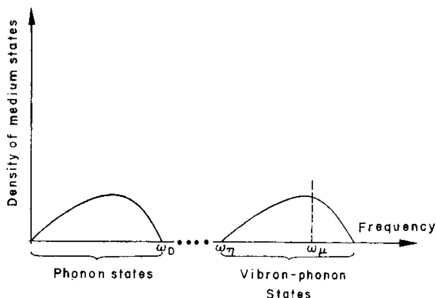
Schematic density of states in a phonon-vibron system. \omega_D is the Debye frequency of phonons; \omega_\eta is the vibron frequency. \omega_\mu corresponds to an intramolecular frequency of a guest molecule.
