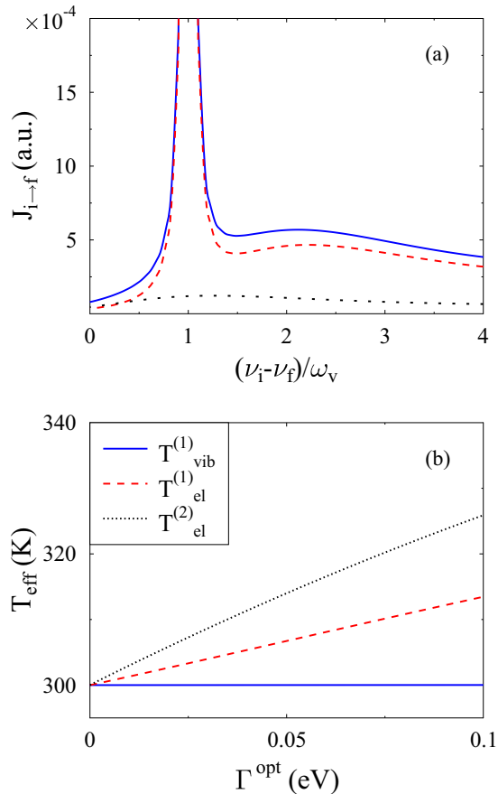
FIG. 6. The Raman scattering signal calculated for model B (see text for parameters). (a) The pure-electronic (black dotted line) and electronic-dressed vibrational Raman (red dashed line) and their sum (full line, blue). (b) The corresponding vibrational and electronic effective temperatures.
