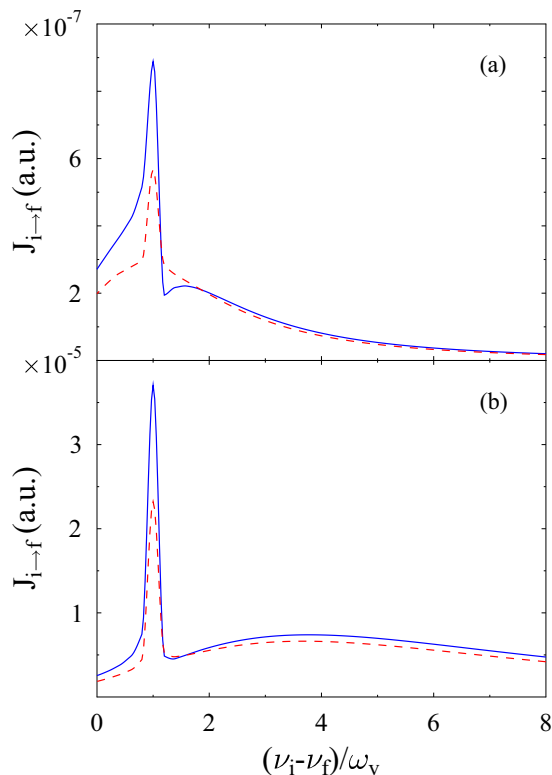
FIG. 4. The Raman scattering (blue solid line) evaluated from Eqs. (S10)–(S16), displayed against the Raman shift \nu_i - \nu_f . The parameters used are T = 300 K, \varepsilon_g = 0 , \varepsilon_x = 2 eV, \Gamma_g = \Gamma_x = 0.05 + \Gamma^{\text{opt}} eV, with \Gamma^{\text{opt}} being the light-induced tunneling rate, \omega_v = 0.05 eV, M_g = 0.02 eV, and \nu_i = 1 eV. The red dashed line is the result obtained when the e-v interaction (6) is disregarded. Shown are results for (a) weak ( \Gamma^{\text{opt}} = 0.03 eV, U^{(0)} = 0.032 eV, U^{(1)} = 0.0032 eV) and (b) strong ( \Gamma^{\text{opt}} = 0.3 eV, U^{(0)} = 0.1 eV, U^{(1)} = 0.01 eV) incident field.
