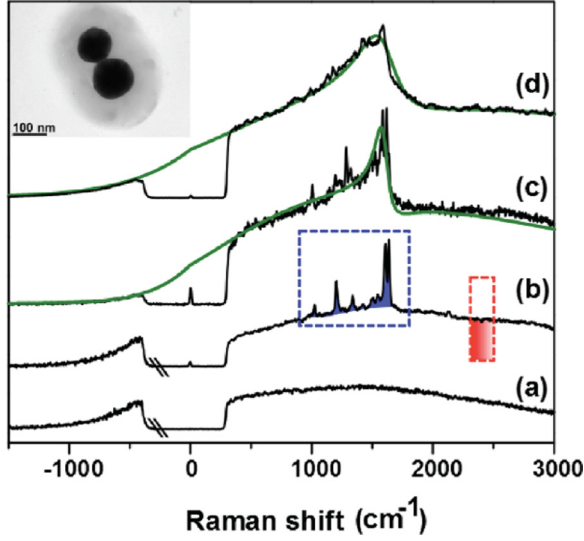
FIG. 1. Raman spectrum recorded on (a) a bare dumbbell, without reporter molecules at low irradiation intensity ( \sim 10 \mu\text{W}/\mu\text{m}^2 ), (b) a dumbbell with reporter molecules at the same low intensity, and a dumbbell with reporter molecules at irradiation intensities of (c) \sim 50 \mu\text{W}/\mu\text{m}^2 and (d) 150 \mu\text{W}/\mu\text{m}^2 . Demarcations on lines (a) and (b) indicate a magnification of the anti-Stokes (AS) region ( 7\times and 4.5\times , respectively). The green traces overlapping lines (c) and (d) are fits to the Fano lineshape (see SI). The blue and red rectangles are used to quantify the intensity dependence of the molecular lines (blue) and electronic Raman scattering of gold (red). The latter leads to results shown in Fig. 2. The inset shows a TEM image of a typical dumbbell.
