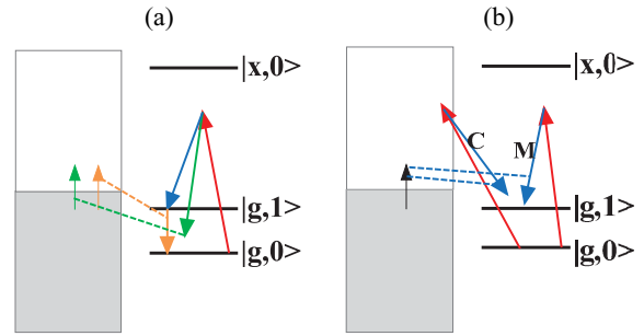
FIG. 3. A sketch of the processes underlying the Stokes (S) component of Raman scattering from a molecule coupled to a metal. (a) The incident photons induce the virtual transition (red) and a corresponding Rayleigh scattering (the red process in reverse). In addition two inelastic scattering (Raman) pathways are shown: electronic Raman scattering (green), which brings the molecule to its ground state while creating an e - h excitation in the metal, and vibrational Raman scattering (blue), which brings the molecule to an excited vibrational state on the electronic ground state. These Raman scattering pathways are coupled by the combined effect of the metal-molecule electron transfer and the electronic-vibrational ( e - v ) interaction (orange) that induces vibrational deexcitation in the molecule with e - h formation in the metal (dashed lines). (b) Two pathways are defined by the excitation process (red): a virtual molecular transition (M) and a molecule-to-metal charge transfer transition (C). The outgoing photon (blue) leaves the molecule in the excited vibrational state, possibly with e - h (de)excitation in the metal (black). The processes shown are also accompanied by electronic Raman scattering from the bare metal.
