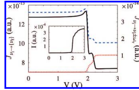
Figure 1. The integrated Raman signal \bar{J}_{\nu_i \rightarrow \{\nu_j\}} (solid line, black, left vertical axis), its Stokes \bar{J}_{\nu_i \rightarrow \nu_i - \omega_\nu} (dashed line, blue, right vertical axis) and anti-Stokes \bar{J}_{\nu_i \rightarrow \nu_i + \omega_\nu} (dotted line, red, right) components, and the current I (inset) displayed as functions of the applied bias V . The parameters used are \nu_i = \bar{\varepsilon}_2 - \bar{\varepsilon}_1 , E_F = 0 , \bar{\varepsilon}_1 = -1 eV, \bar{\varepsilon}_2 = 1 eV, \omega_\nu = 0.1 eV, \Omega_\nu = 0.005 eV, V_1^{(\text{e-v})} = 0.1 eV, V_2^{(\text{e-v})} = 0.05 eV and T = 100 K, “a.u.” denotes atomic units.
