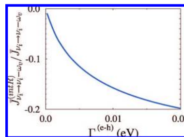
Figure 3. The ratio between the interference component and the total Raman flux at the Stokes frequency, \bar{J}_{\nu_i \rightarrow \nu_i - \omega_\nu}^{(\text{int})} / \bar{J}_{\nu_i \rightarrow \nu_i - \omega_\nu} , at V = 2.5 V as a function of \Gamma^{(e-h)} for \Gamma_m = 0.01 eV and \nu_i = \Delta\varepsilon . Other parameters as in Figure 2.
