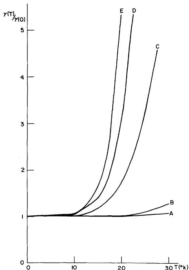
FIG. 1. Model calculations for the temperature dependence of the vibrational relaxation rate of a guest diatomic molecule in a monatomic lattice. A: \omega = 1000 \text{ cm}^{-1} , \omega_A = 100 \text{ cm}^{-1} ; B: \omega = 3000 \text{ cm}^{-1} , \omega_A = 100 \text{ cm}^{-1} ; C: \omega = 1000 \text{ cm}^{-1} , \omega_A = 50 \text{ cm}^{-1} ; D: \omega = 2000 \text{ cm}^{-1} , \omega_A = 50 \text{ cm}^{-1} ; E: \omega = 3000 \text{ cm}^{-1} , \omega_A = 50 \text{ cm}^{-1} .
