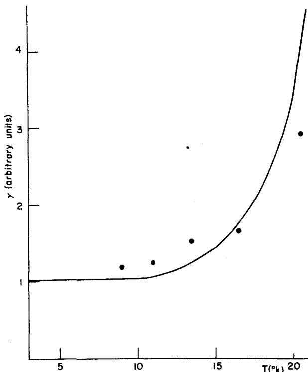
FIG. 2. The temperature dependence of the vibrational relaxation rate of CO in solid Ar. \bullet : Experimental data of Legay, Abouaf-Marguin, and Dubost [Refs. (7-9)]. These relative values can be converted into absolute values taking \gamma = 73 \text{ sec}^{-1} at T = 9^\circ \text{K} ; —: Theoretical curve from Eq. (30), with \omega = 2170 \text{ cm}^{-1} and \omega_A = 50 \text{ cm}^{-1} .
