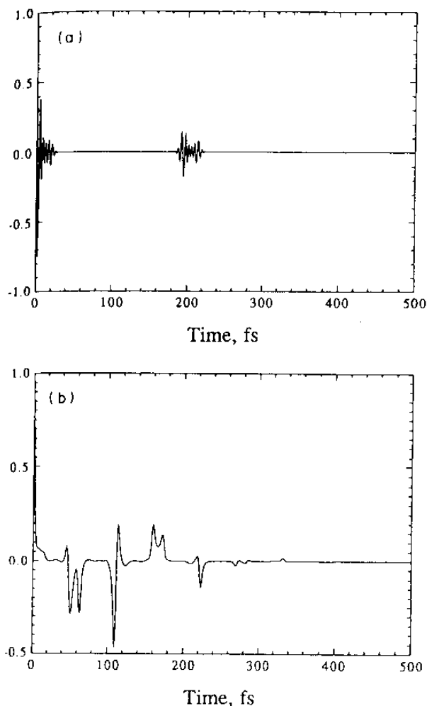
Fig. 8. Reduced-dimension treatment for the (a) HMB/TCNE and (b) Ru/Fe charge transfer systems. Here, the many-mode systems have been approximated by two modes, one high-frequency and one low-frequency, plus a single (frequency, 1 \text{ cm}^{-1} ; reorganization energy, 2300 \text{ cm}^{-1} ) solvent mode. Integrals are (a) 0.121 \text{ fs} and (b) 5.89 \text{ fs} . (See text and Fig. 5.)
