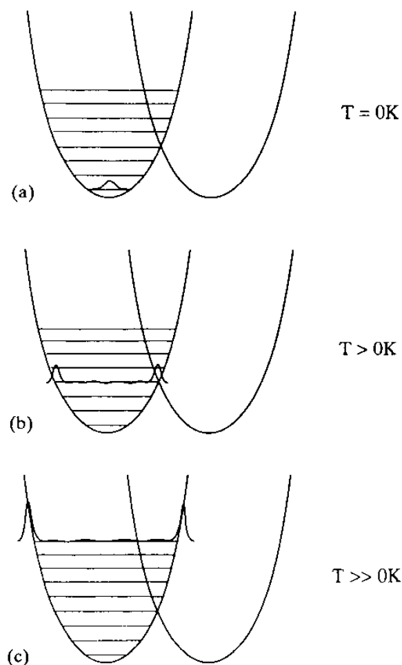
Fig. 12. Pictorial description of temperature effects on rate in a degenerate system. At T=0\text{ K} (a), only the n=0 vibrational level is populated, and Franck-Condon overlaps are small. At T>0 (b), levels closer to the crossing point become populated and the average rate increases. As higher levels become populated ( T \gg 0 ) (c), the rate drops again, as higher vibrational levels again have smaller Franck-Condon overlaps with the final surface. The curves depicted are sketches of \langle Y^2 \rangle .
