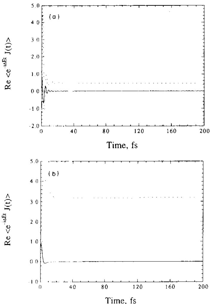
Fig. 5. \langle \exp[-i\Delta E t] J(t) \rangle for (a) the HMB/TCNE and (b) the Ru/Fe charge transfer systems, with both 200 \text{ cm}^{-1} inhomogeneous gap modulation and a 1 \text{ cm}^{-1} solvent mode ( \lambda_{\text{sol}} = 2300 \text{ cm}^{-1} ) added (see text). Integrals are (a) 0.272 fs and (b) 4.46 fs. Trajectories are chosen at T = 0 \text{ K} . Solid lines represent the averaged integrand \langle \exp[-i\Delta E t] J(t) \rangle , while the broken line is a running sum of the integrand (as seen in ^1\text{H} NMR plots, for example). Note that the integral is unchanging after 50 fs in both cases; see Table 2 for integrated rates.
