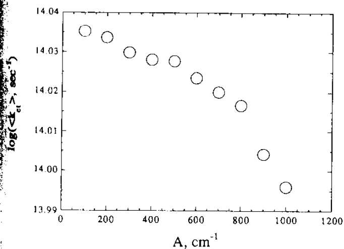
Fig. 9. Dependence of averaged rate ( T=0 \text{ K} ) on gap modulation constant A (see text) for the Ru/Fe charge transfer system.
