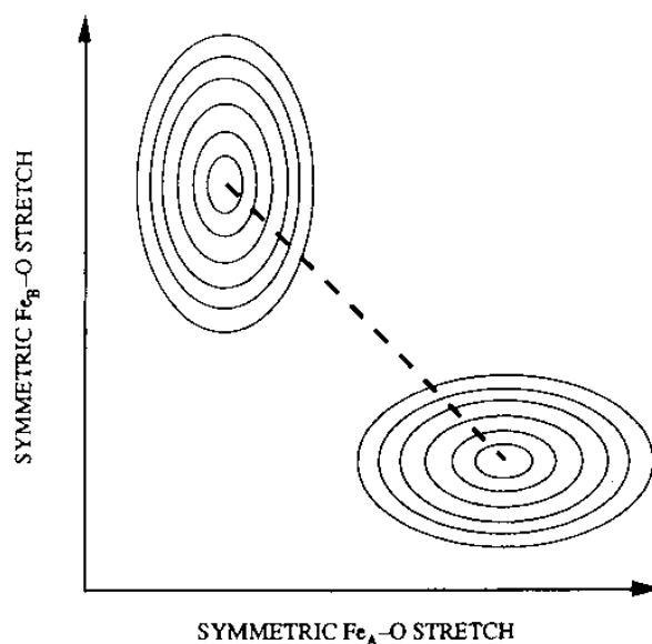
Fig. 7. Pictorial description of the hexa-aquo-iron ( 2+/3+ ) exchange reaction (characteristic frequencies: 389 and 490 \text{ cm}^{-1} ; see Table 1). When the electron is transferred, there are frequency changes corresponding to changes in oxidation states of the iron centers. Siders and Marcus have approximated this mode system by a single energy-weighted average system of mode ( 431 \text{ cm}^{-1} ). Then the reaction coordinate is given by broken line (see text and Fig. 6). Here, the differences in frequency have been over-emphasized for clarity.
