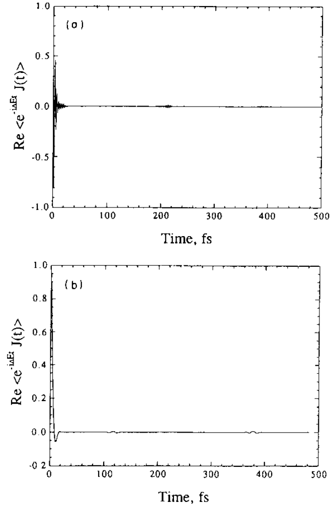
Fig. 4. \langle \exp[-i\Delta Et]J(t) \rangle for (a) the HMB/TCNE and (b) the Ru/Fe charge transfer systems, with 200\text{ cm}^{-1} of inhomogeneous electronic gap modulation added (see text and Fig. 3). These represent the average of 200 trajectories (sufficient to give convergence of C(t) ), with trajectories chosen at T = 0\text{ K} .
