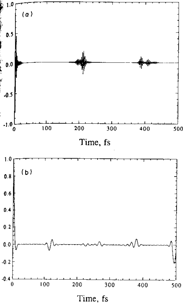
Fig. 3. \exp(-i\Delta Et)J(t) for (a) the HMB/TCNE ( \Delta E_{IF} = 11\,600\text{ cm}^{-1} ; V_{IF} \approx 3500\text{ cm}^{-1} ; \lambda_i = 3515\text{ cm}^{-1} ) and (b) the Ru/Fe charge transfer systems ( \Delta E_{IF} = 3000\text{ cm}^{-1} ; V_{IF} \approx 3200\text{ cm}^{-1} ; \lambda_i = 3220\text{ cm}^{-1} ) (see text). These are single trajectories, with T = 0\text{ K} .
