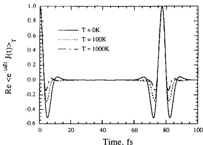
Fig. 11. Comparison of integrands of the one-mode ( 431\text{ cm}^{-1} ) system of Fig. 2 at 0, 100, and 1000\text{ K} (see text) (200 trajectories). Note that the width and amplitude of the recurrences are narrowed at higher temperatures.
