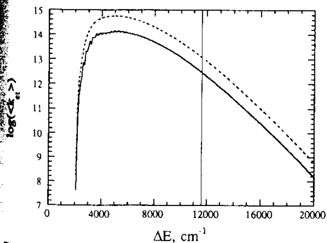
Fig. 10. \log\langle k_{\text{et}} \rangle ( \text{s}^{-1} ) vs. \Delta E for the HMB/TCNE charge transfer system, with an additional 1 \text{ cm}^{-1} (solvent) mode with \lambda_{\text{sol}}=3900 \text{ cm}^{-1} (from Markel et al. [13]) and 200 \text{ cm}^{-1} inhomogeneous gap modulation. Solid line represents the time-dependent golden-rule (TDGR) formulation, while the broken line represents the steepest-descents (SD) method of Fischer and van Duyne (see text and ref. 8). The vertical line represents the experimentally measured \Delta E for this system. (The noise associated with the TDGR treatment is the result of numerical integration error.)
