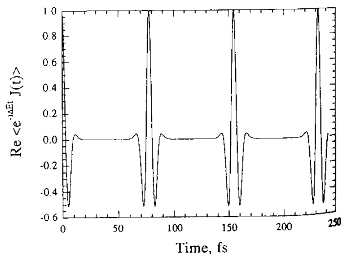
Fig. 2. \exp[-i\Delta Et]J(t) for the model Fe ( 2+/3+ ) system described in the text and Table 1. J(t) here is as defined in eqn. (4b), thus, in this and subsequent figures, the vertical axis is unitless. Relevant parameters for the one-mode case shown are as follows: \hbar\omega = 431 \text{ cm}^{-1} ; \lambda_i = 2926 \text{ cm}^{-1} ; \Delta E_{IF} = 0 ; T = 0 \text{ K} . Note that, because of the absence of irreversible processes, we observe recurrence
