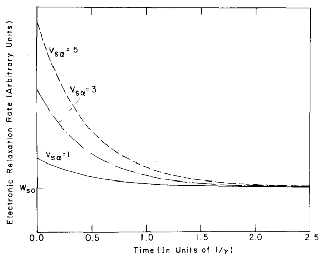
FIG. 2. Electronic relaxation rate as a function of time [Eq. (VII.6)], for a model molecule characterized by 30 randomly chosen frequencies ( \omega chosen between 500 \text{ cm}^{-1} and 3000 \text{ cm}^{-1} ) and by origin shifts \Delta_\mu=1 for every vibrational mode. The electronic energy gap was taken as 12\,000 \text{ cm}^{-1} . The molecule is assumed to be initially in the excited vibronic state |s, V_{s\alpha}, \{0_\mu\}_{\mu \neq \alpha}\rangle . At long times the decay rate approaches W_{s0} , the decay rate of the vibrationless level of the s th electronic manifold.
